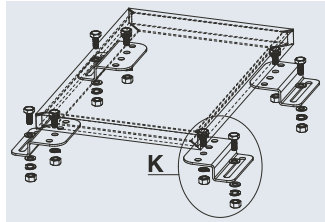
CSLB-0120 – Side of Pole/Wall Mount Bracket
